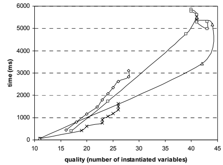
Figure 5. Relation between runtime and quality of solution for RCSP \langle 50,12, 250/1225,0.35 \rangle , \diamond -CS, \square -DBS, \triangle -IB, \times -LAN.
