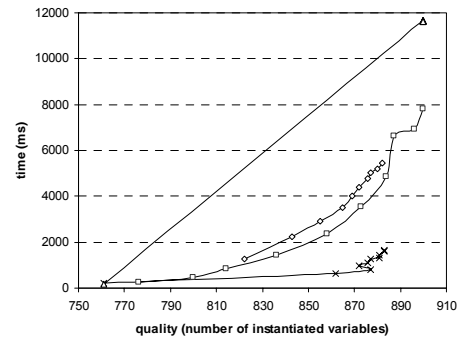
Figure 6. Relation between runtime and quality of solution for QWH, order 30 and 40% holes, \diamond -CS, \square -DBS, \triangle -IB, \times -LAN.
